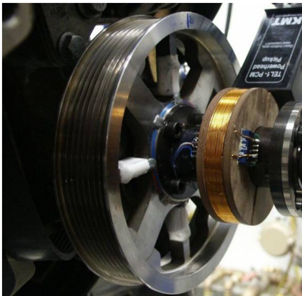
Half capsulated housing on shaft
