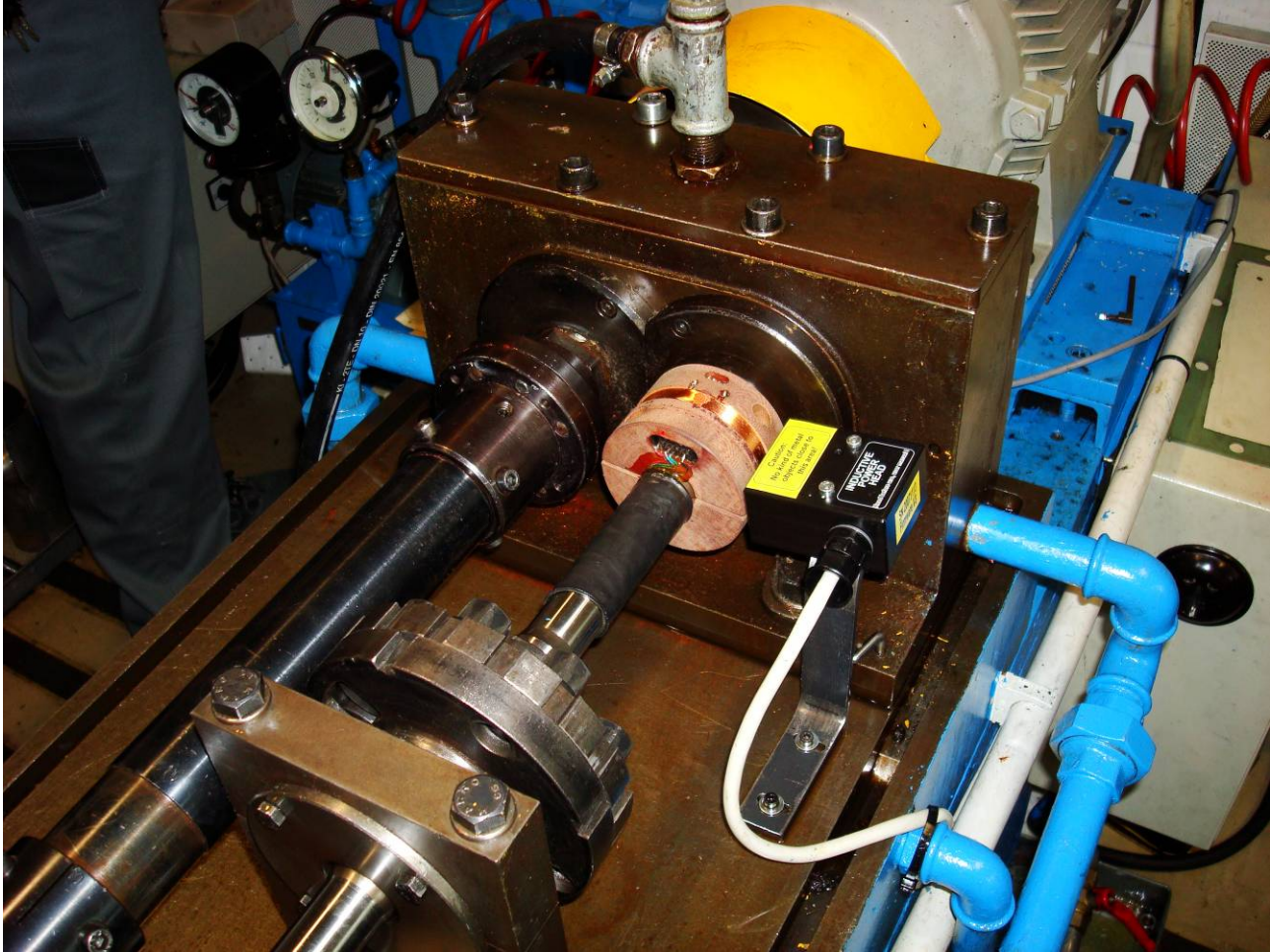
Complete capsulated housing on shaft
