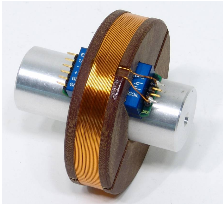
Half capsulated housing on shaft
