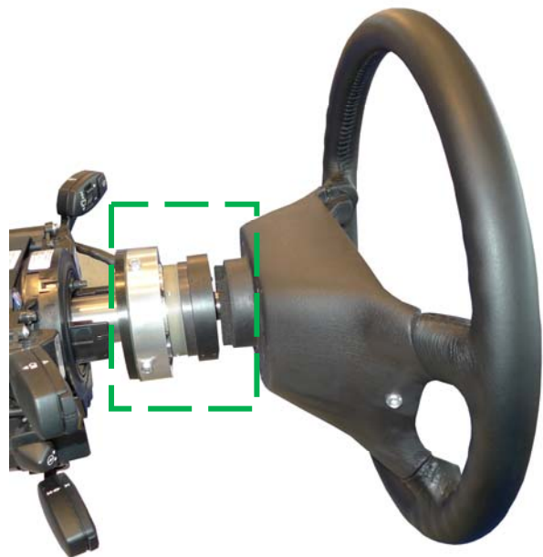
KMT-CLS Sensor in a standard application, located between steering wheel and steering column
